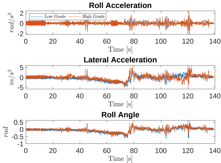
Figure 7: Low and high grade IMU sensor outputs.
